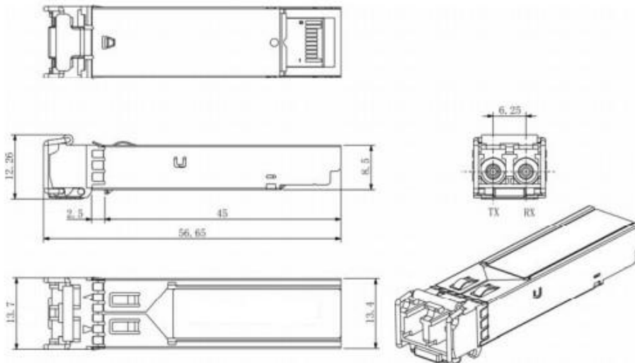
Mechanical Drawing
